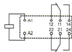
2 FORM C (DPDT)
